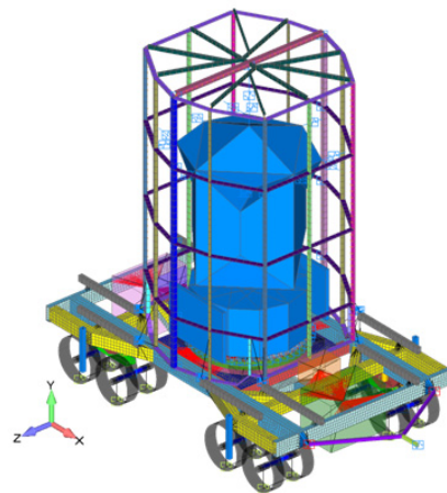
▲ Finite element model of the Cygnus Vertical Container
