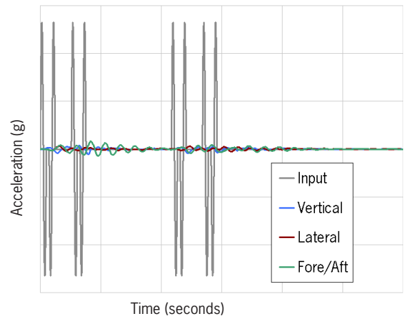
▲ Isolated time history response of Cygnus spacecraft during transport
