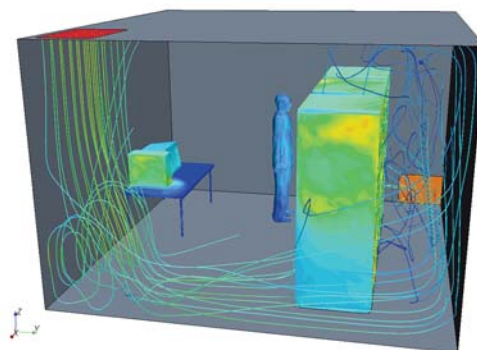
▲ Overview of an electronic equipment room. The flow from the top left vent is colored by velocity (red = higher, blue = lower velocity). The server racks, person, and computer table are colored by temperature (red = higher, blue = lower temperature).
