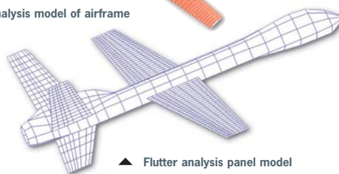
▲ Detailed finite element analysis model of airframe
